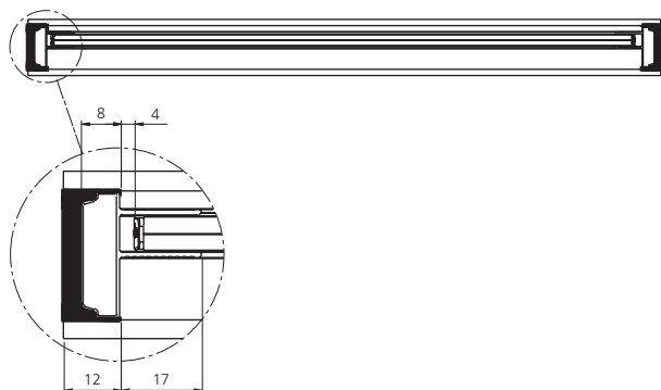
EXTRUDED "U" SPACER BAR 27X8 mm WITH 17 mm GUIDE PROJECTION
