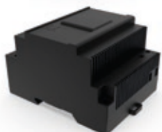
SL2712 Rev. 1 Switching Power Supply 24V dc 2.5 A DIN rail mounting Dim.: 3 modules 52.5x90x54.5 mm (WxHxD)
